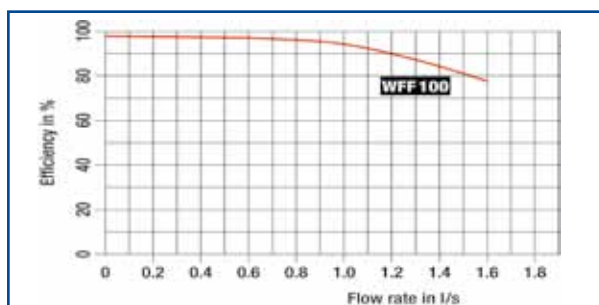
Efficiency rate curve for Vortex Fine Filter WFF 100. Measurements taken from a newly fabricated filter.
